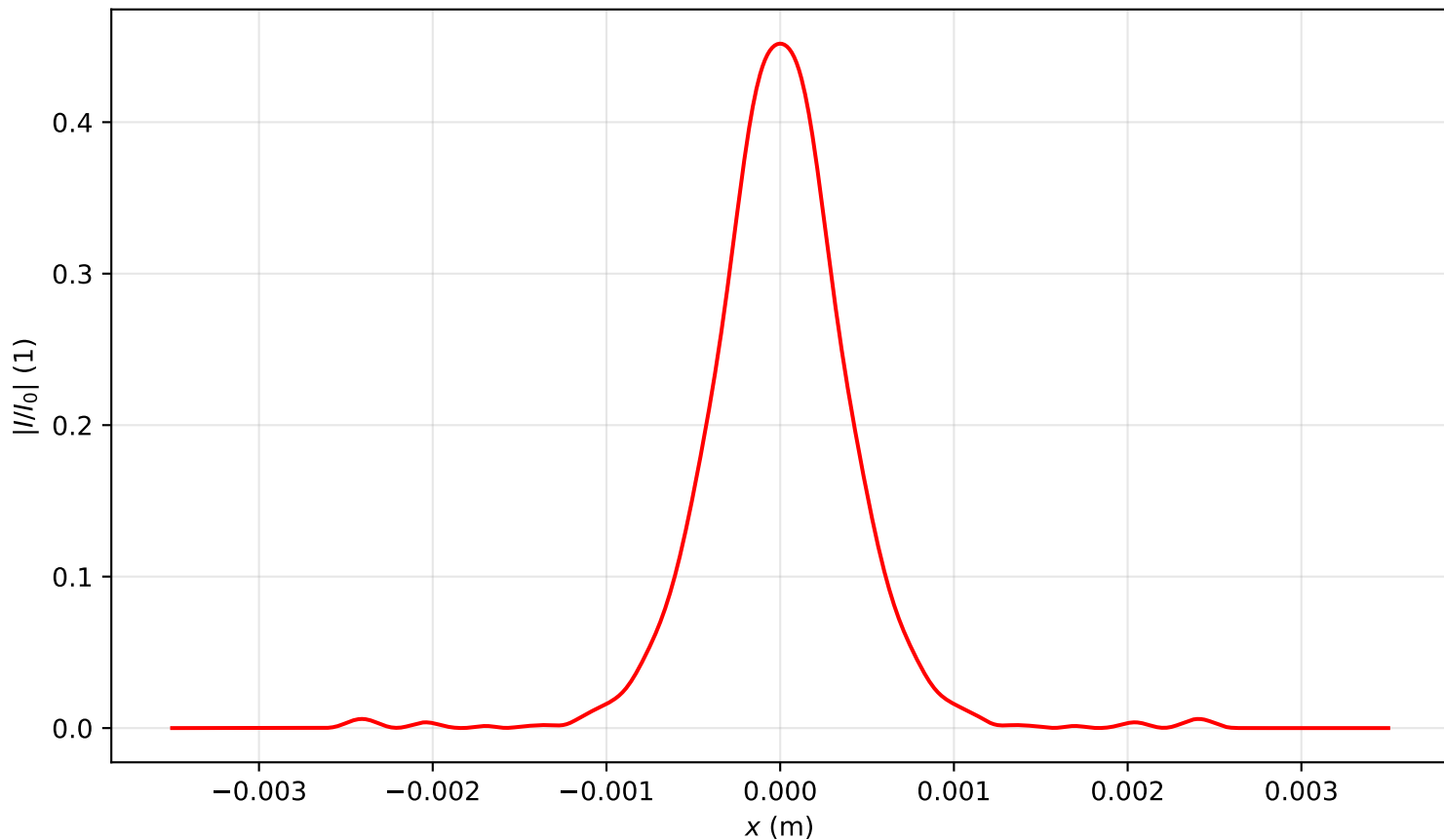
Intensity profile I(x, y = 0, z = 2.388)/I_0 , P_{in}=1.0P_{cr} , artificial time
